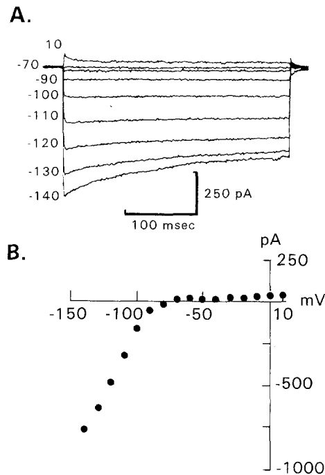
Fig. 1. (A) Inwardly rectifying K current. Cell was held at -70 mV and 440 msec voltage pulses applied in 10-mV increments. Records have not been leak subtracted to show total current. (B) Peak current-voltage plot for experiment shown in A
