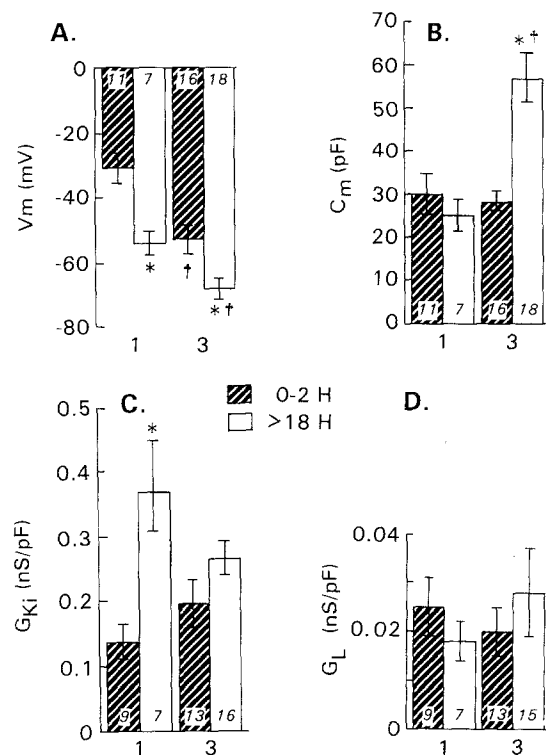
Fig. 6. (A) V_m , (B) C_m , (C) G_{K_i} , and (D) G_L with time after adherence for round (group 1) and spread (group 3) cells. Mean values were compared at 0–2 and >18 hr for each group. *Indicates values that are significantly different from values from the same group at 0–2 hr. †Indicates values that are significantly different from values of group 1 at the same time period
