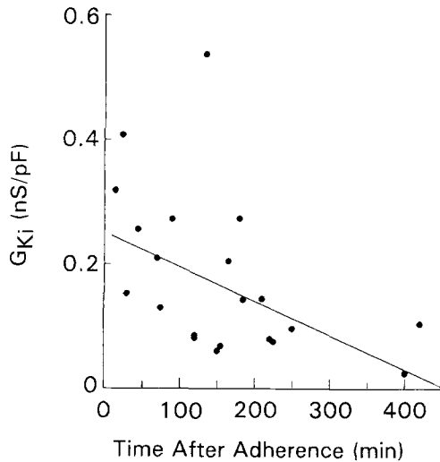
Fig. 4. Plot of G_{K_i} vs. time after adherence for cycloheximide-treated cells. Solid line is a linear biweight fit to the data. Its slope is significantly different from zero. Note that cells were exposed to cycloheximide 1 hr prior to plating, as well as during plating
